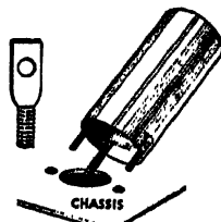
Spade bolt and typical use.
